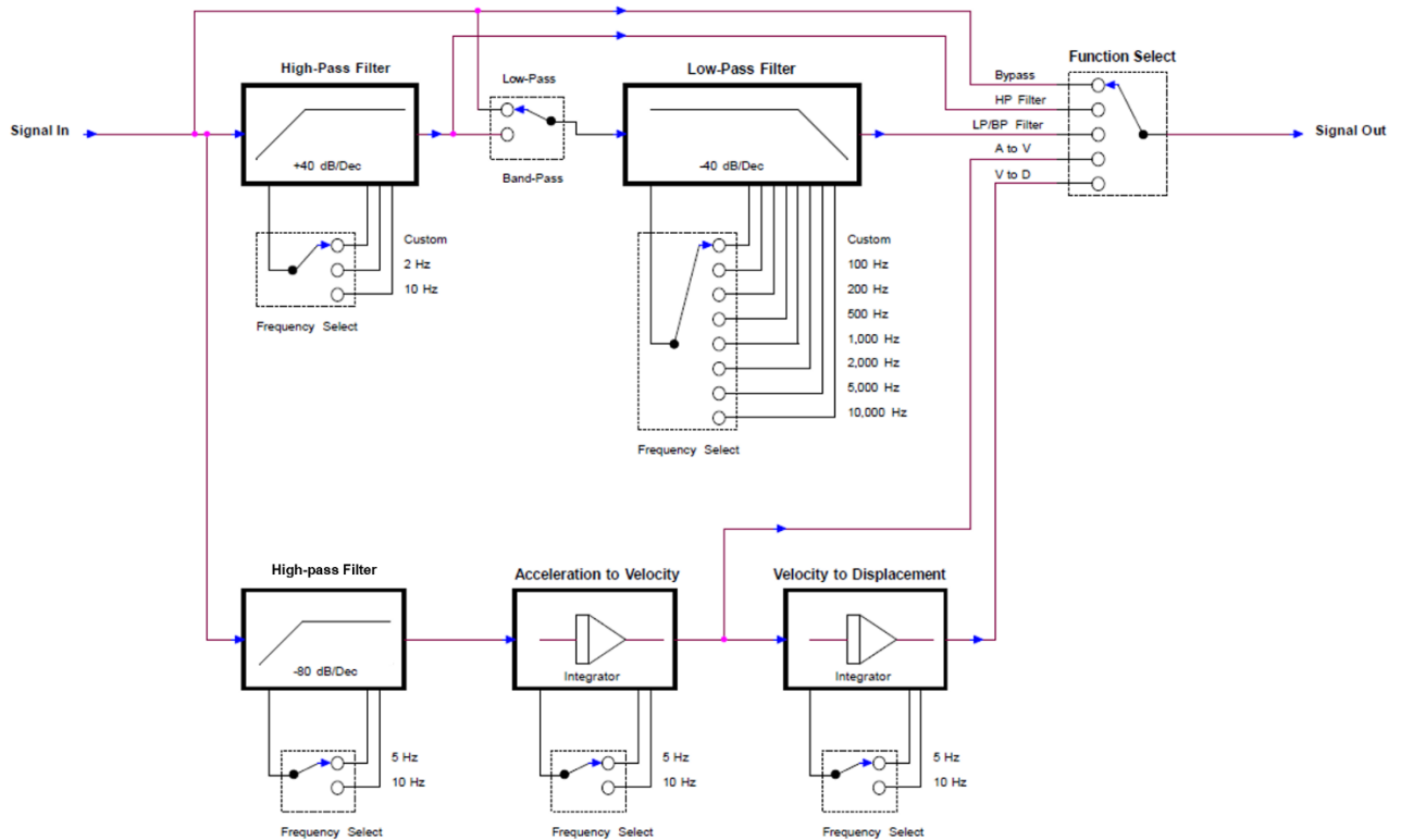
Figure 10: Filter block diagram
