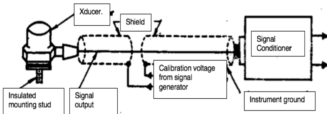
Figure 23: T-Junction wiring diagram
